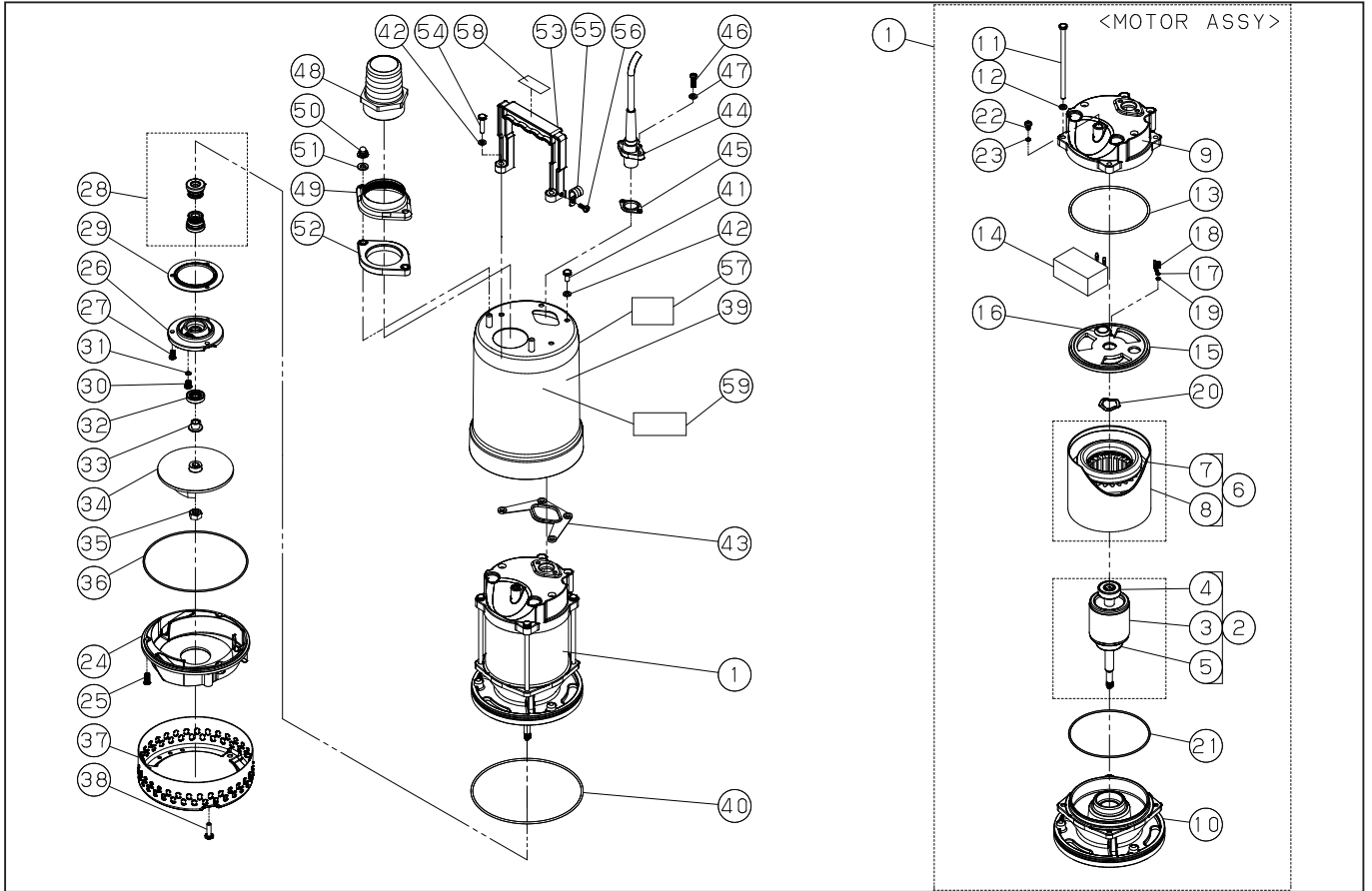
DWG No.077850201 MODELE : PXJ-250 FORM : PXJ-250-BAB-0
